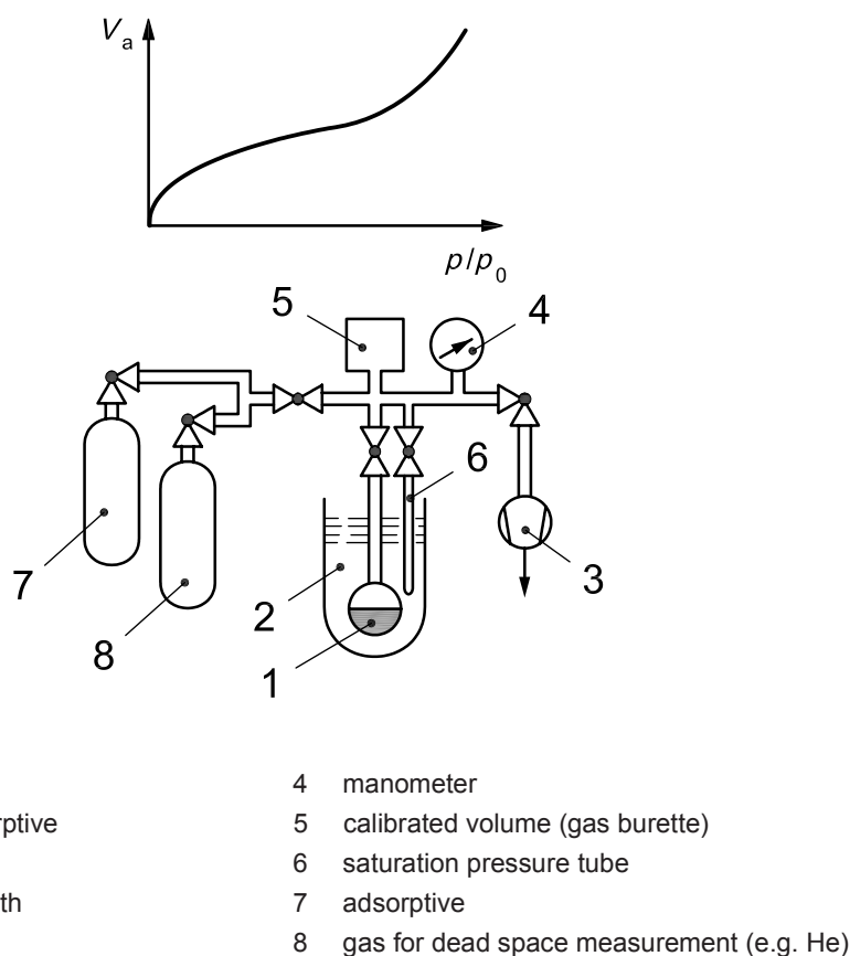
Figure 6 — Volumetric method
